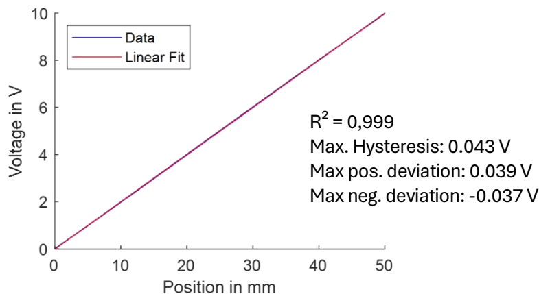
Figure 1: Typical sensor data (three cycles) and the linear fit
