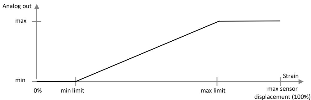
Figure 3: Analog output signal with taught limits.
