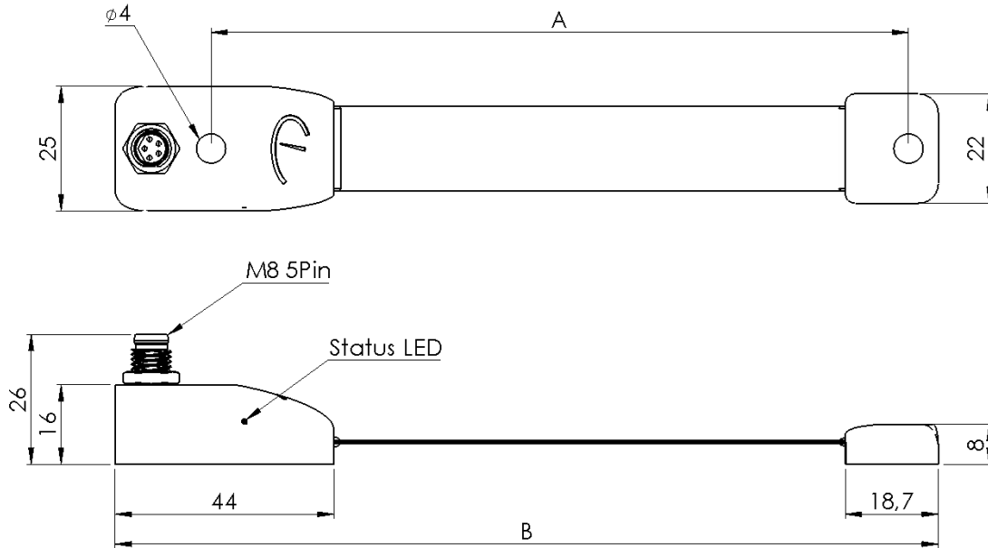
Figure 2: Drawing of Sensor
